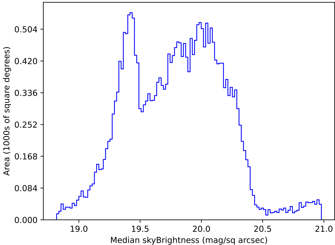
too_elab_r32_d2_ugrizy_v3.4_10yrs Yr 1 all bands: Median skyBrightness
