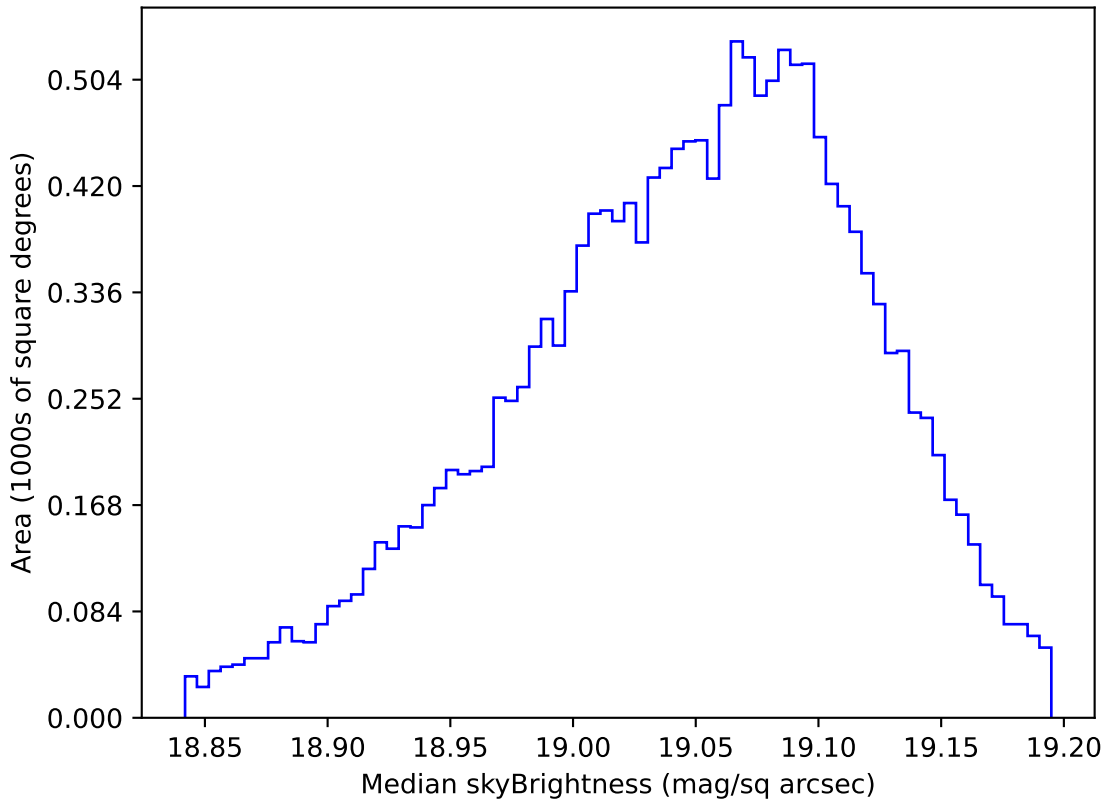
too_elab_r32_d2_ugrizy_v3.4_10yrs WFD z band: Median skyBrightness
