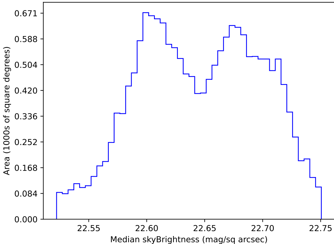
too_elab_r32_d2_ugrizy_v3.4_10yrs WFD u band: Median skyBrightness
