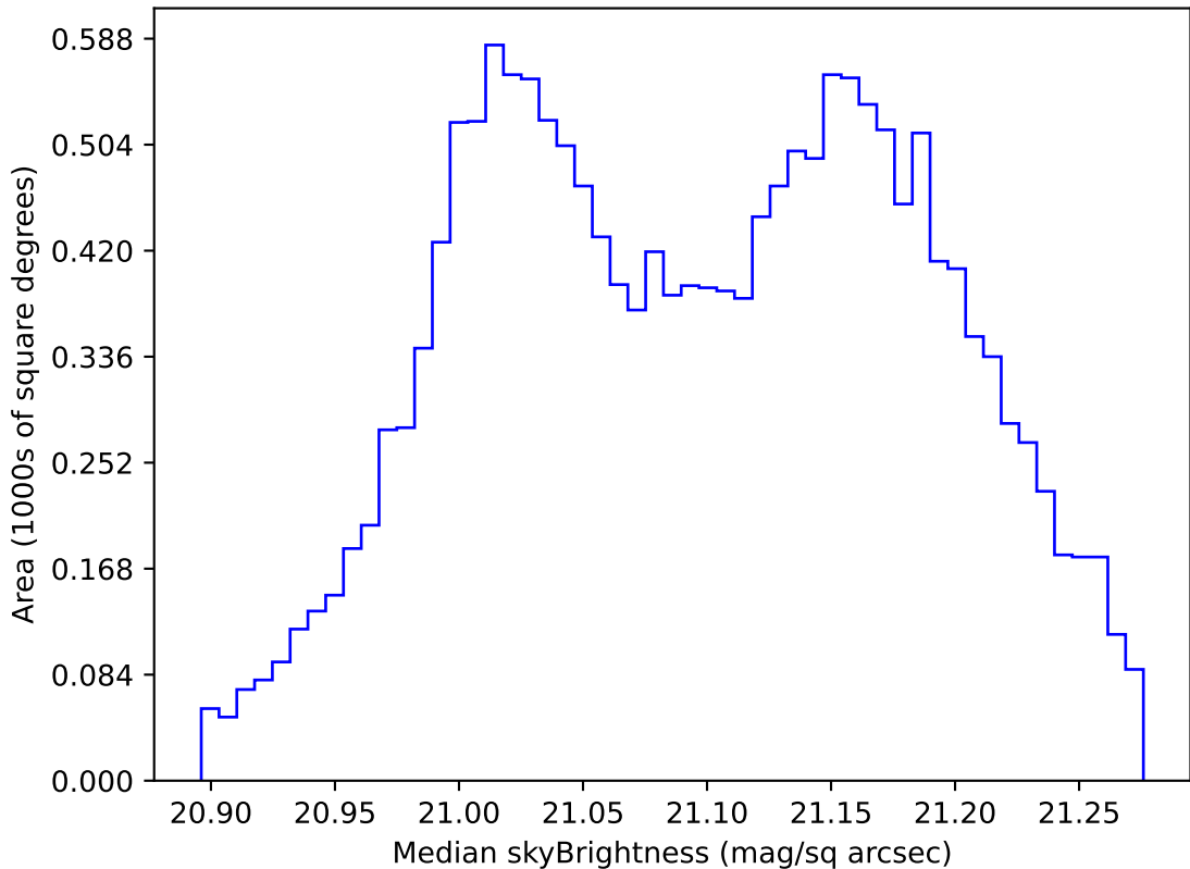
too_elab_r32_d2_ugrizy_v3.4_10yrs WFD r band: Median skyBrightness
