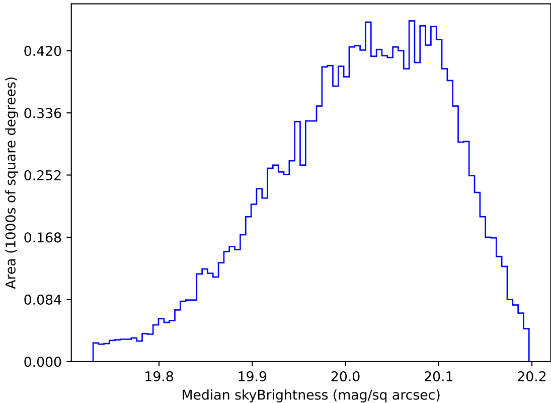
too_elab_r32_d2_ugrizy_v3.4_10yrs WFD i band: Median skyBrightness
