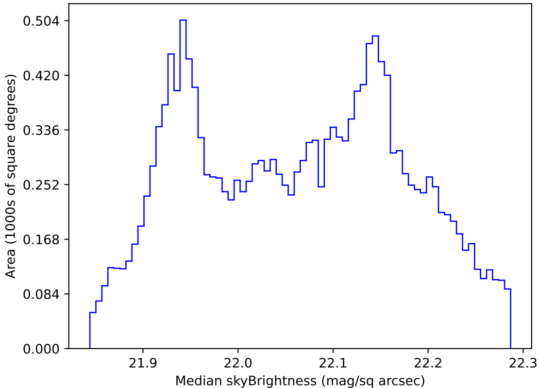
too_elab_r32_d2_ugrizy_v3.4_10yrs WFD g band: Median skyBrightness
