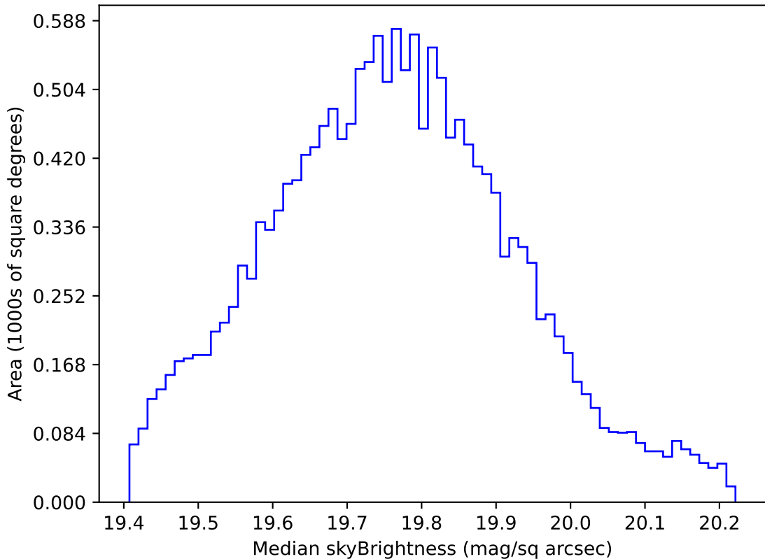
too_elab_r32_d2_ugrizy_v3.4_10yrs WFD all bands: Median skyBrightness
