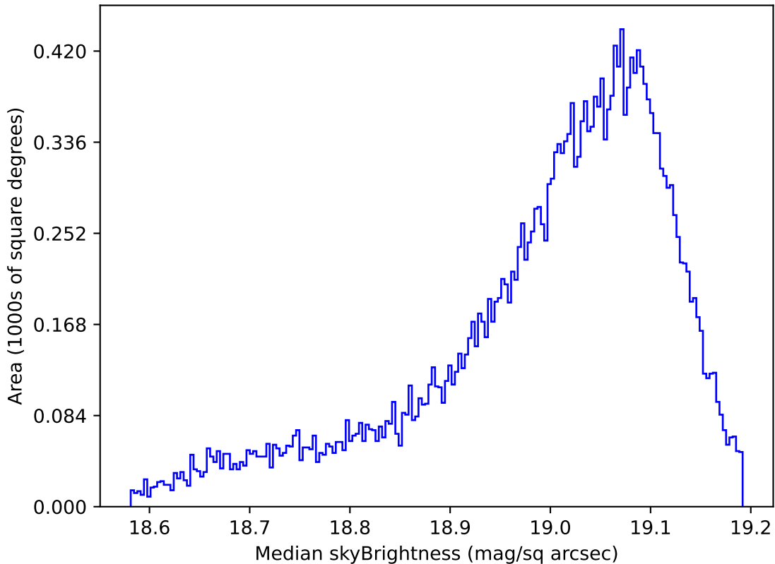
too_elab_r32_d2_ugrizy_v3.4_10yrs All sky z band: Median skyBrightness
