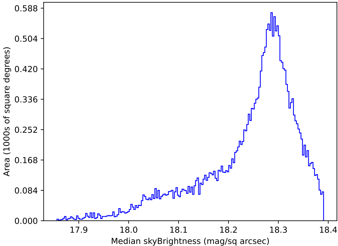
too_elab_r32_d2_ugrizy_v3.4_10yrs All sky y band: Median skyBrightness
