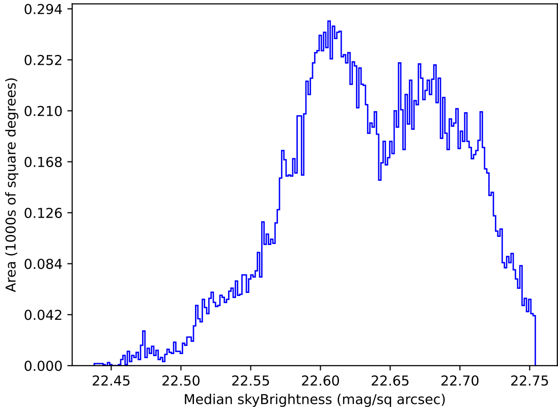
too_elab_r32_d2_ugrizy_v3.4_10yrs All sky u band: Median skyBrightness
