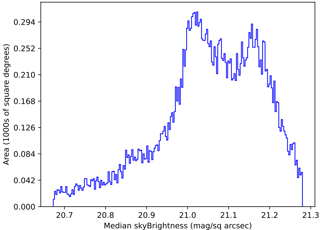
too_elab_r32_d2_ugrizy_v3.4_10yrs All sky r band: Median skyBrightness
