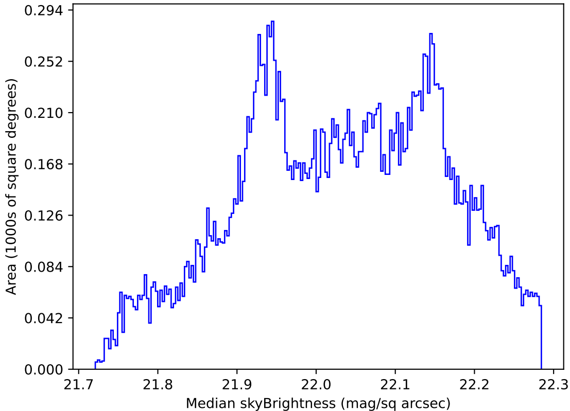
too_elab_r32_d2_ugrizy_v3.4_10yrs All sky g band: Median skyBrightness
