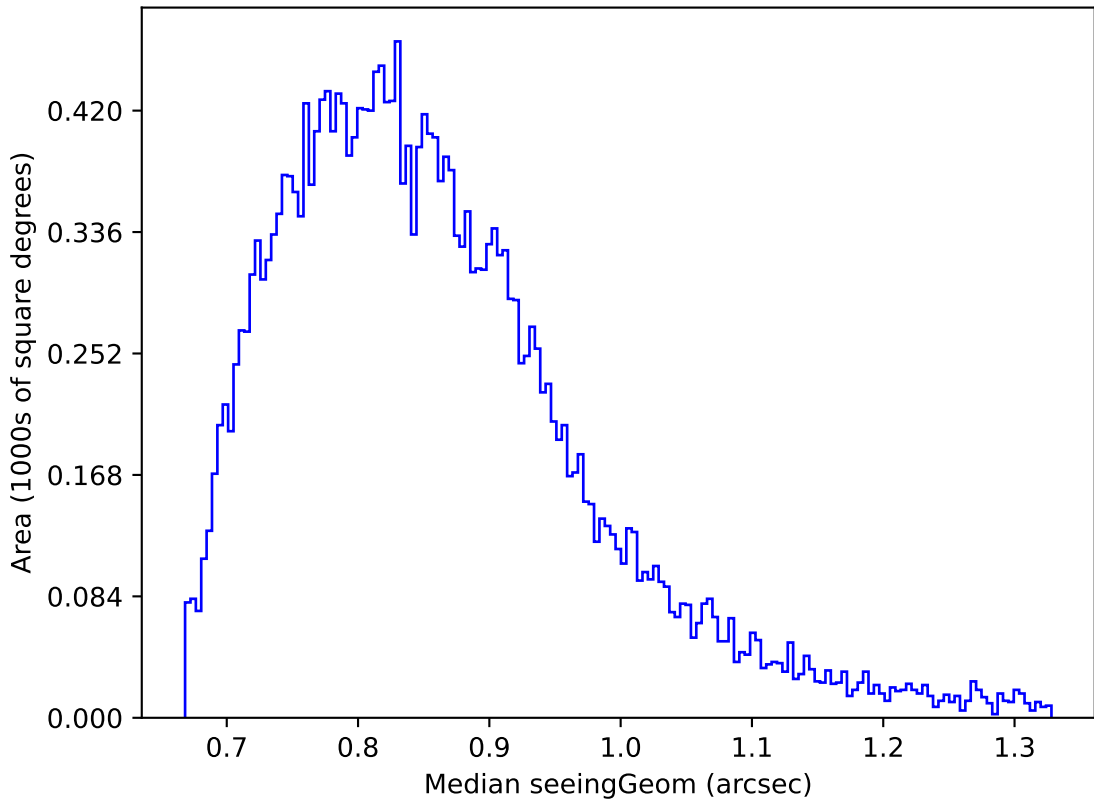
too_elab_r32_d2_ugrizy_v3.4_10yrs Yr 1 z band: Median seeingGeom
