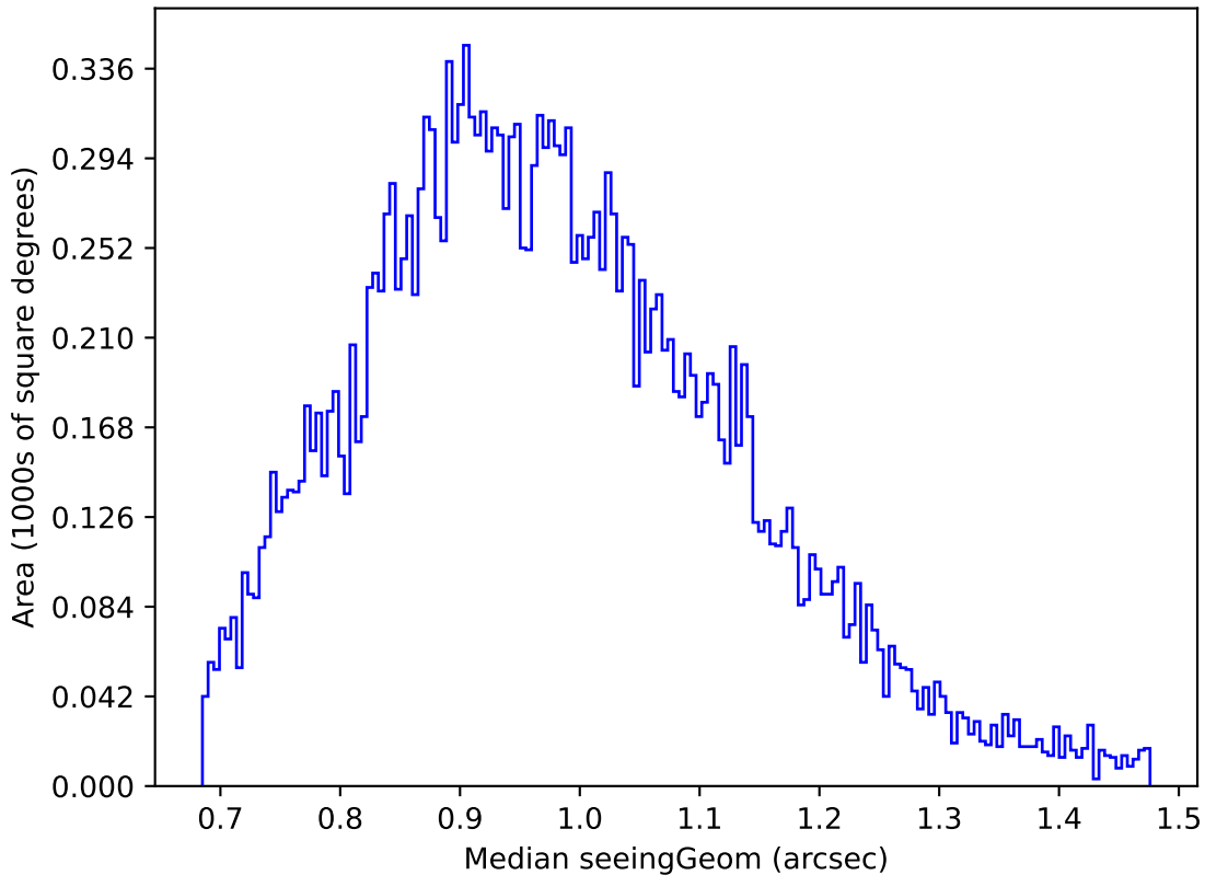
too_elab_r32_d2_ugrizy_v3.4_10yrs Yr 1 u band: Median seeingGeom
