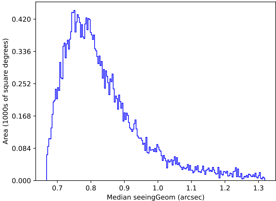
too_elab_r32_d2_ugrizy_v3.4_10yrs Yr 1 i band: Median seeingGeom
