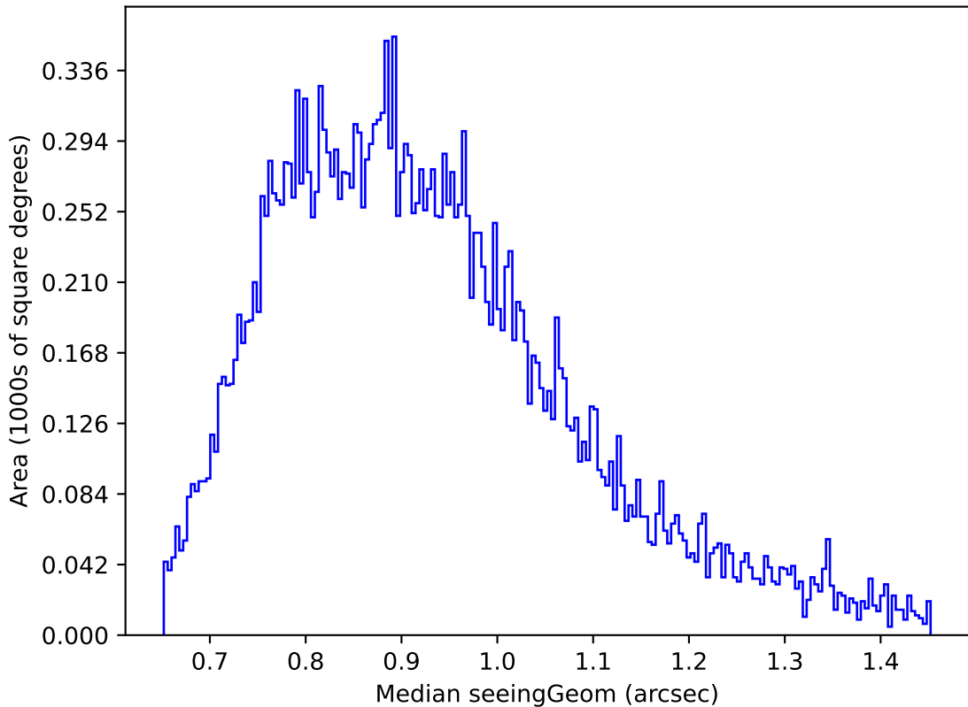
too_elab_r32_d2_ugrizy_v3.4_10yrs Yr 1 g band: Median seeingGeom
