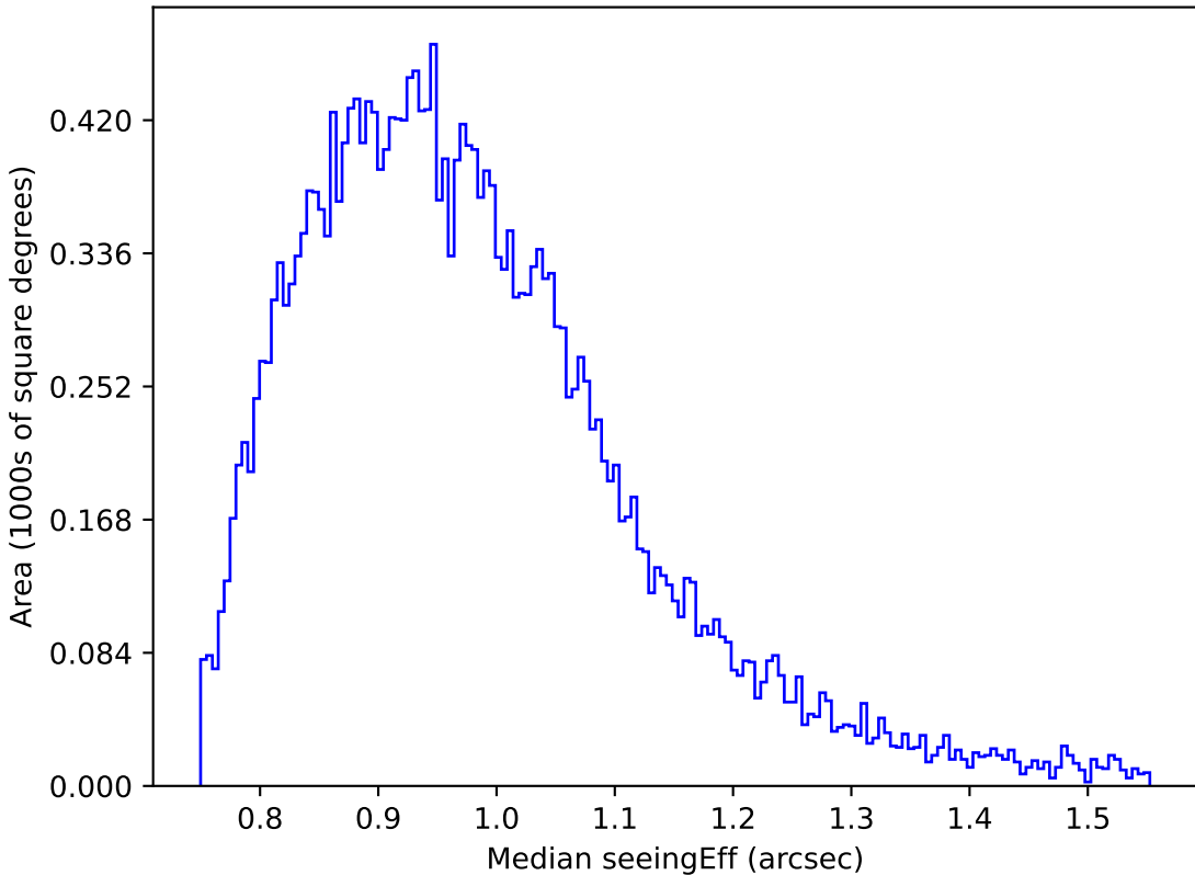
too_elab_r32_d2_ugrizy_v3.4_10yrs Yr 1 z band: Median seeingEff
