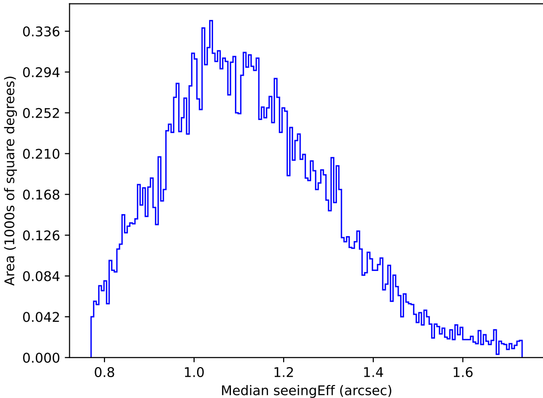
too_elab_r32_d2_ugrizy_v3.4_10yrs Yr 1 u band: Median seeingEff
