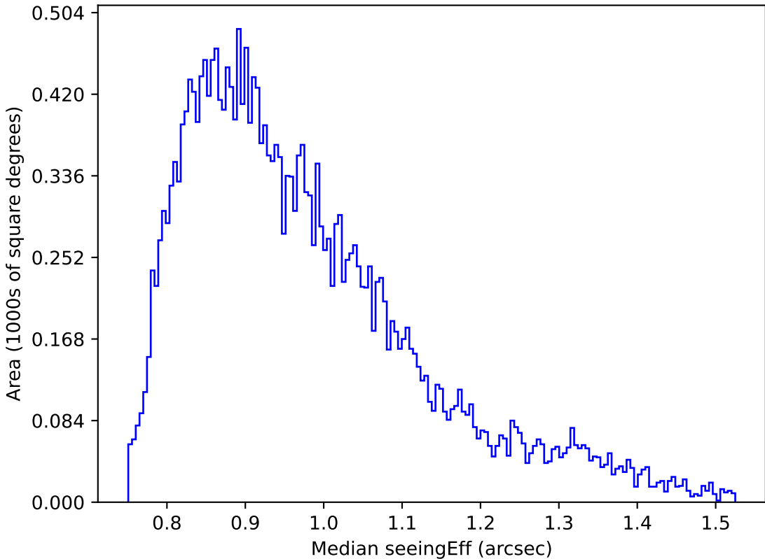
too_elab_r32_d2_ugrizy_v3.4_10yrs Yr 1 r band: Median seeingEff
