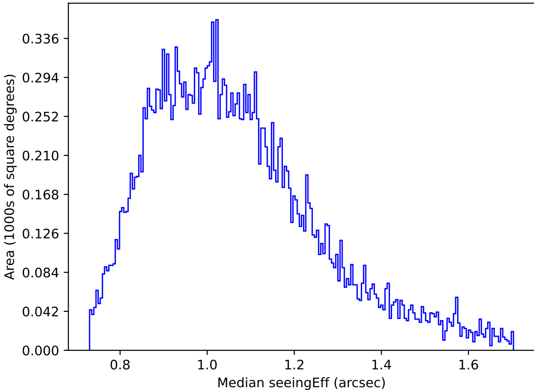
too_elab_r32_d2_ugrizy_v3.4_10yrs Yr 1 g band: Median seeingEff
