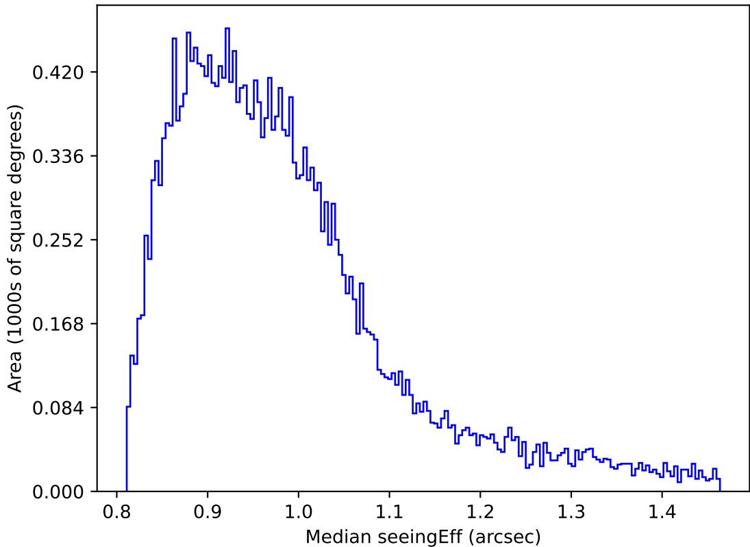
too_elab_r32_d2_ugrizy_v3.4_10yrs Yr 1 all bands: Median seeingEff
