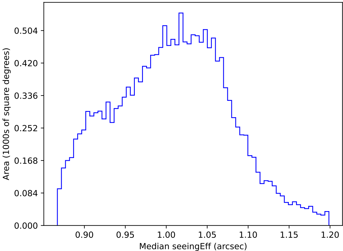
too_elab_r32_d2_ugrizy_v3.4_10yrs WFD z band: Median seeingEff
