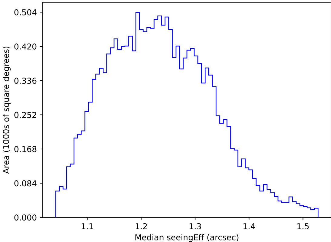
too_elab_r32_d2_ugrizy_v3.4_10yrs WFD u band: Median seeingEff
