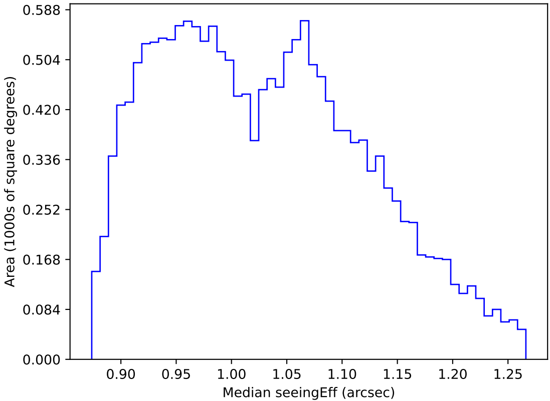
too_elab_r32_d2_ugrizy_v3.4_10yrs WFD r band: Median seeingEff
