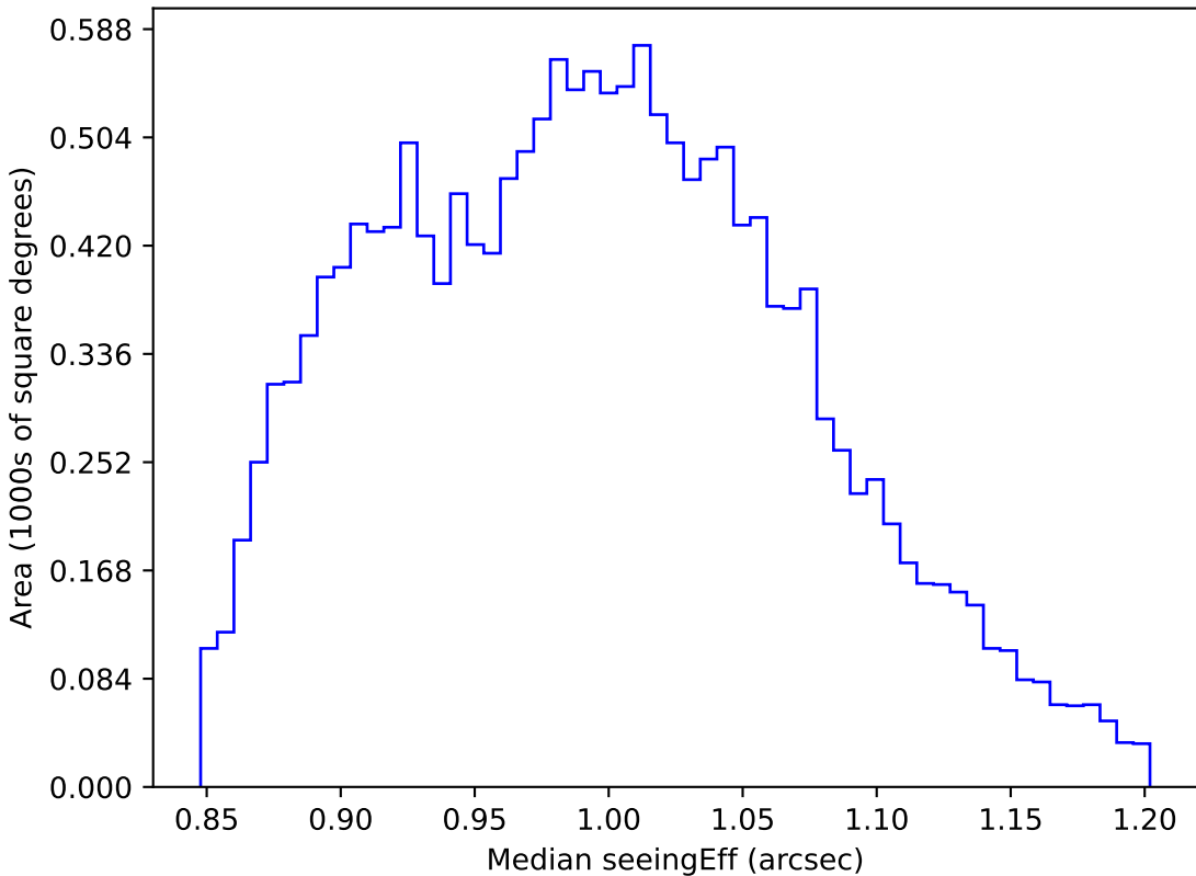
too_elab_r32_d2_ugrizy_v3.4_10yrs WFD i band: Median seeingEff
