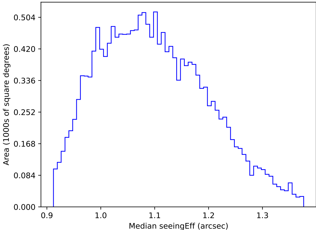
too_elab_r32_d2_ugrizy_v3.4_10yrs WFD g band: Median seeingEff
