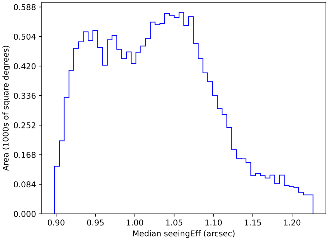
too_elab_r32_d2_ugrizy_v3.4_10yrs WFD all bands: Median seeingEff
