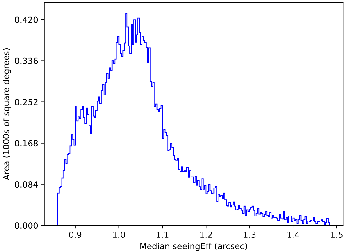
too_elab_r32_d2_ugrizy_v3.4_10yrs All sky z band: Median seeingEff
