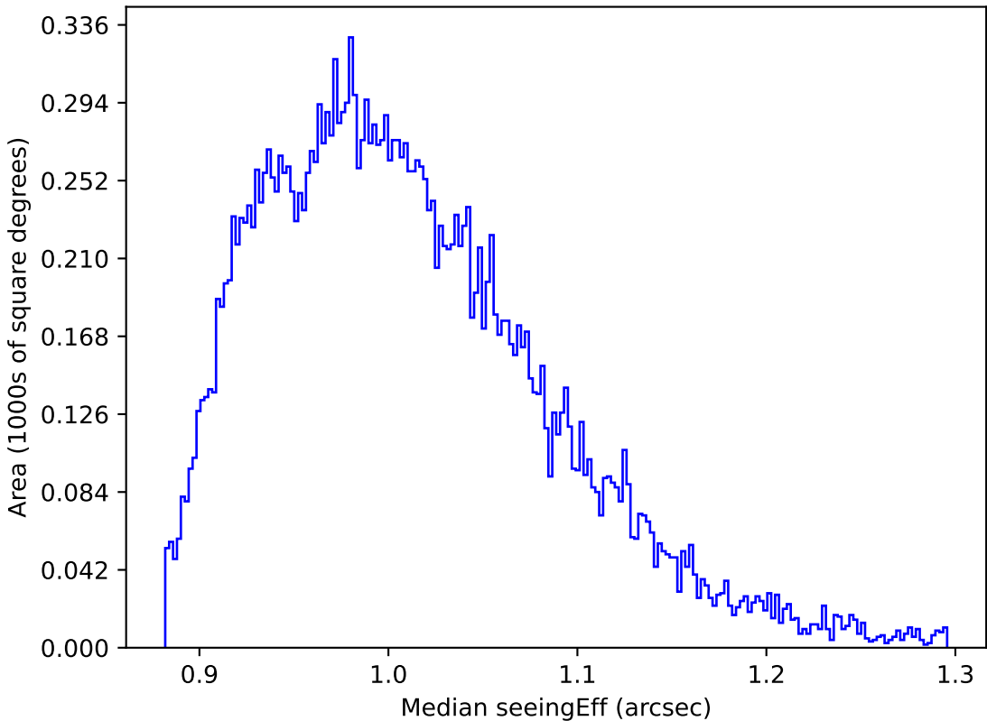
too_elab_r32_d2_ugrizy_v3.4_10yrs All sky y band: Median seeingEff
