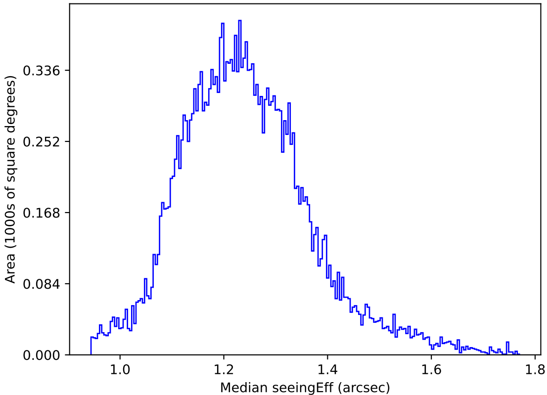
too_elab_r32_d2_ugrizy_v3.4_10yrs All sky u band: Median seeingEff
