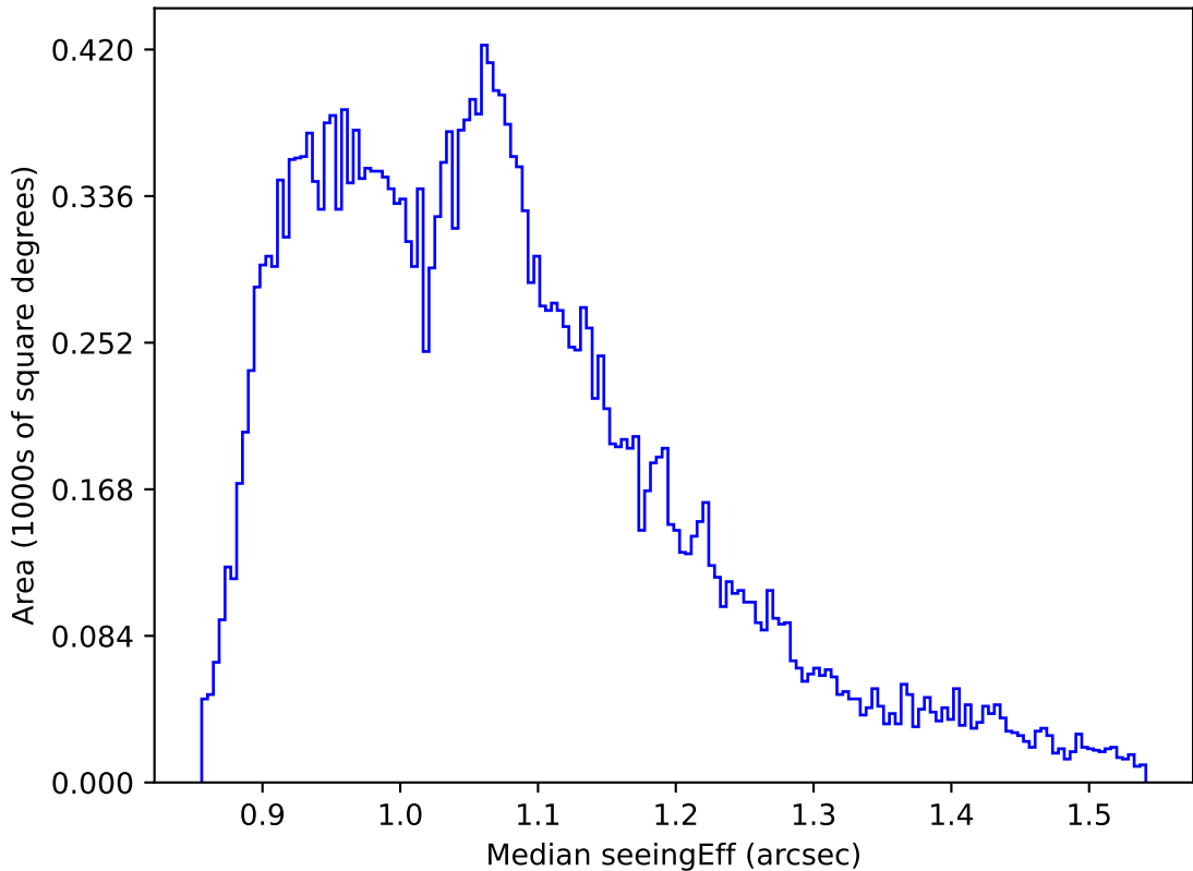
too_elab_r32_d2_ugrizy_v3.4_10yrs All sky r band: Median seeingEff
