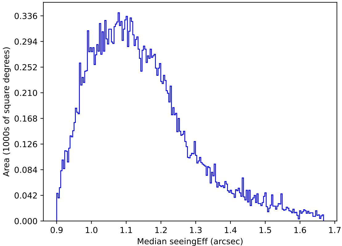
too_elab_r32_d2_ugrizy_v3.4_10yrs All sky g band: Median seeingEff
