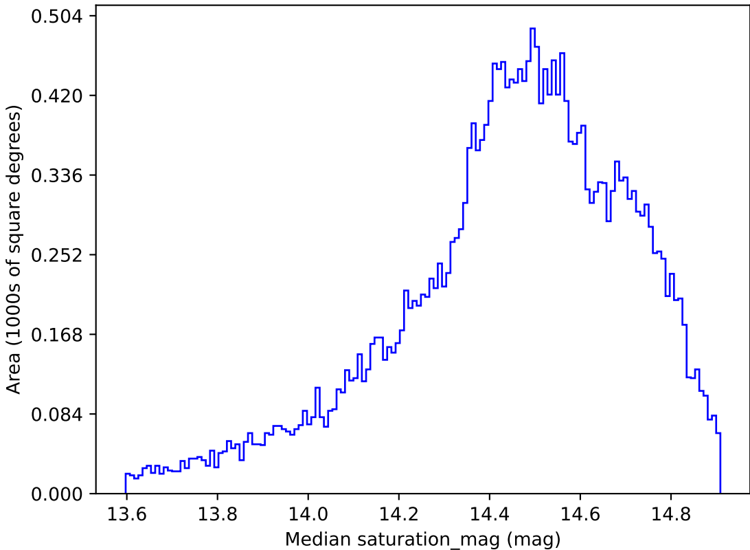
too_elab_r32_d2_ugrizy_v3.4_10yrs All sky i band: Median saturation_mag
