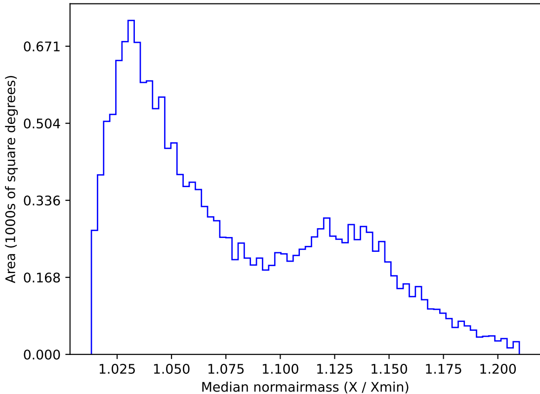
too_elab_r32_d2_ugrizy_v3.4_10yrs WFD u band: Median normairmass
