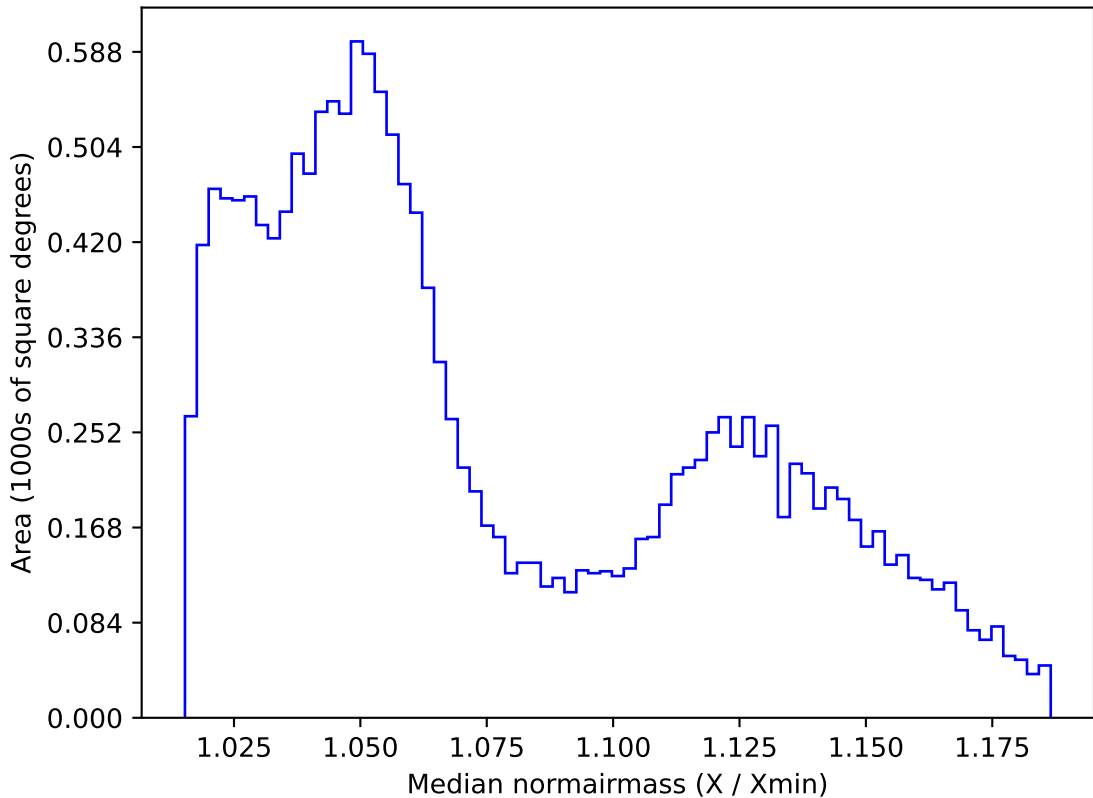
too_elab_r32_d2_ugrizy_v3.4_10yrs WFD r band: Median normairmass
