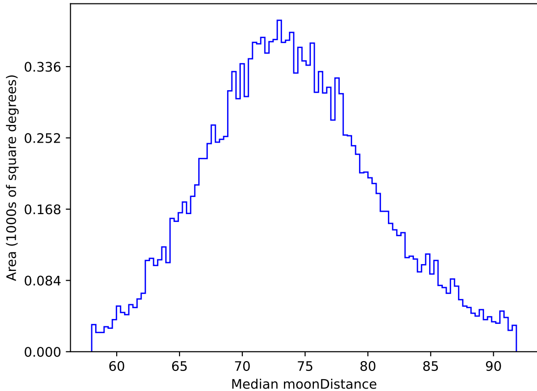
too_elab_r32_d2_ugrizy_v3.4_10yrs WFD z band: Median moonDistance
