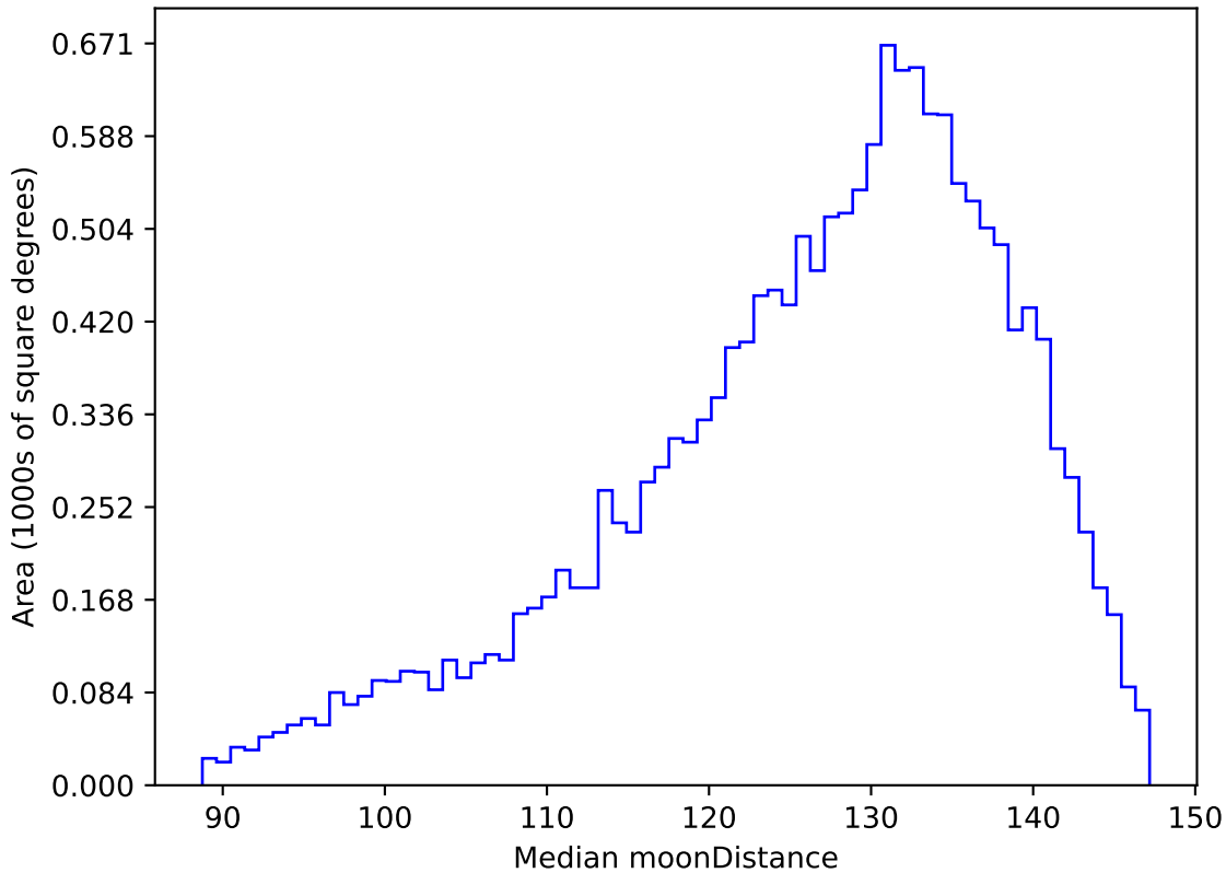
too_elab_r32_d2_ugrizy_v3.4_10yrs WFD u band: Median moonDistance
