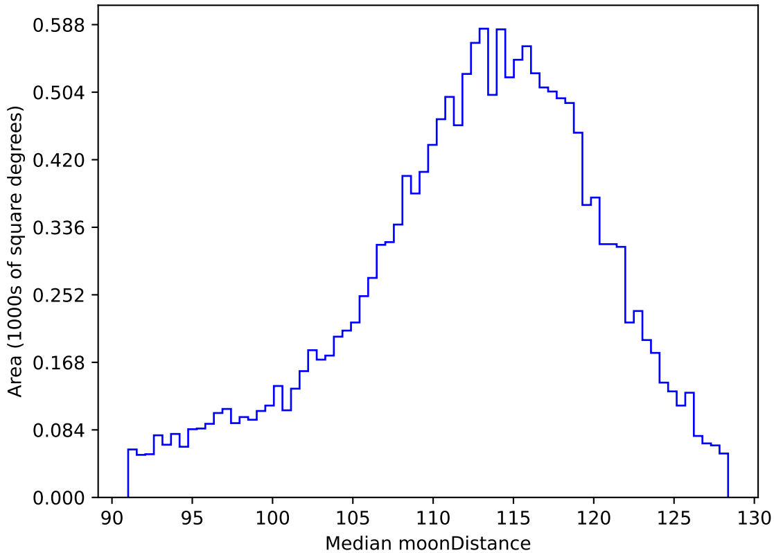
too_elab_r32_d2_ugrizy_v3.4_10yrs WFD r band: Median moonDistance
