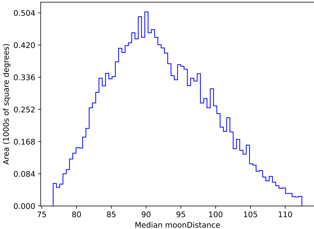
too_elab_r32_d2_ugrizy_v3.4_10yrs WFD i band: Median moonDistance
