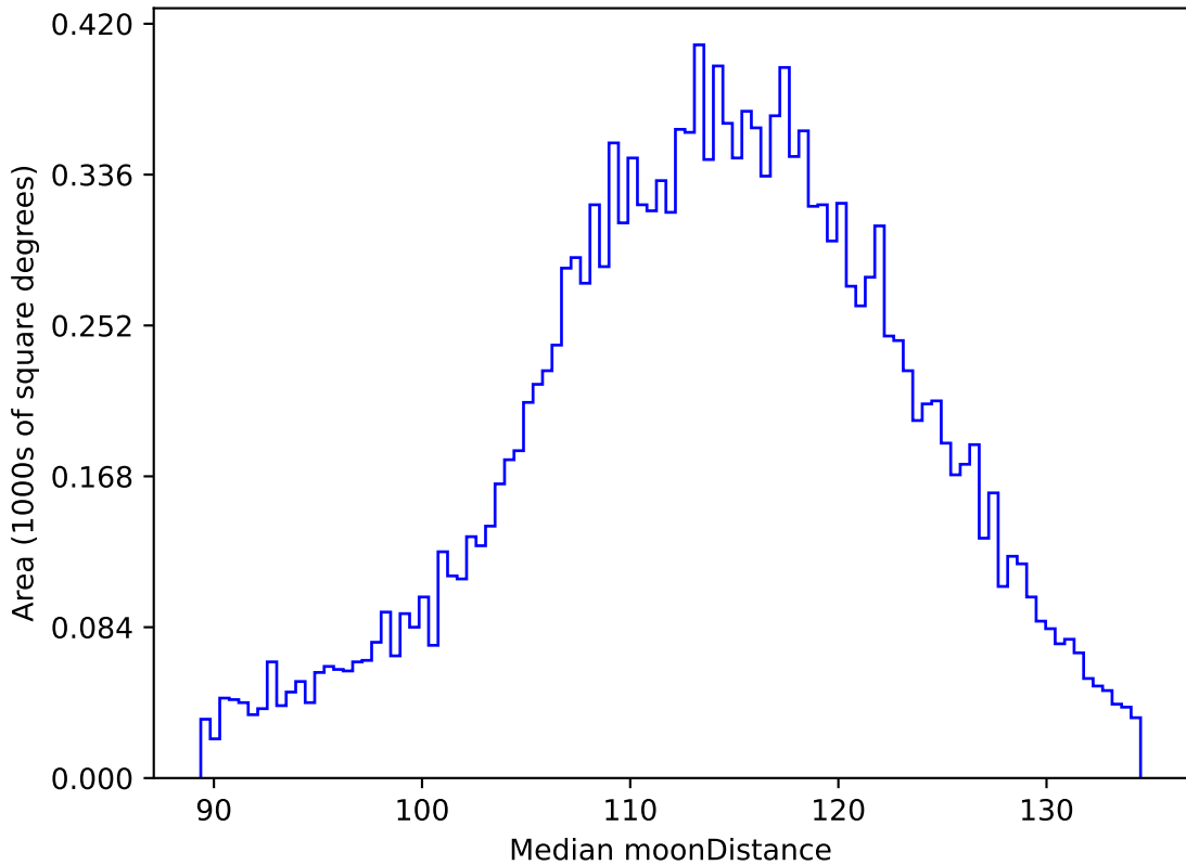
too_elab_r32_d2_ugrizy_v3.4_10yrs WFD g band: Median moonDistance
