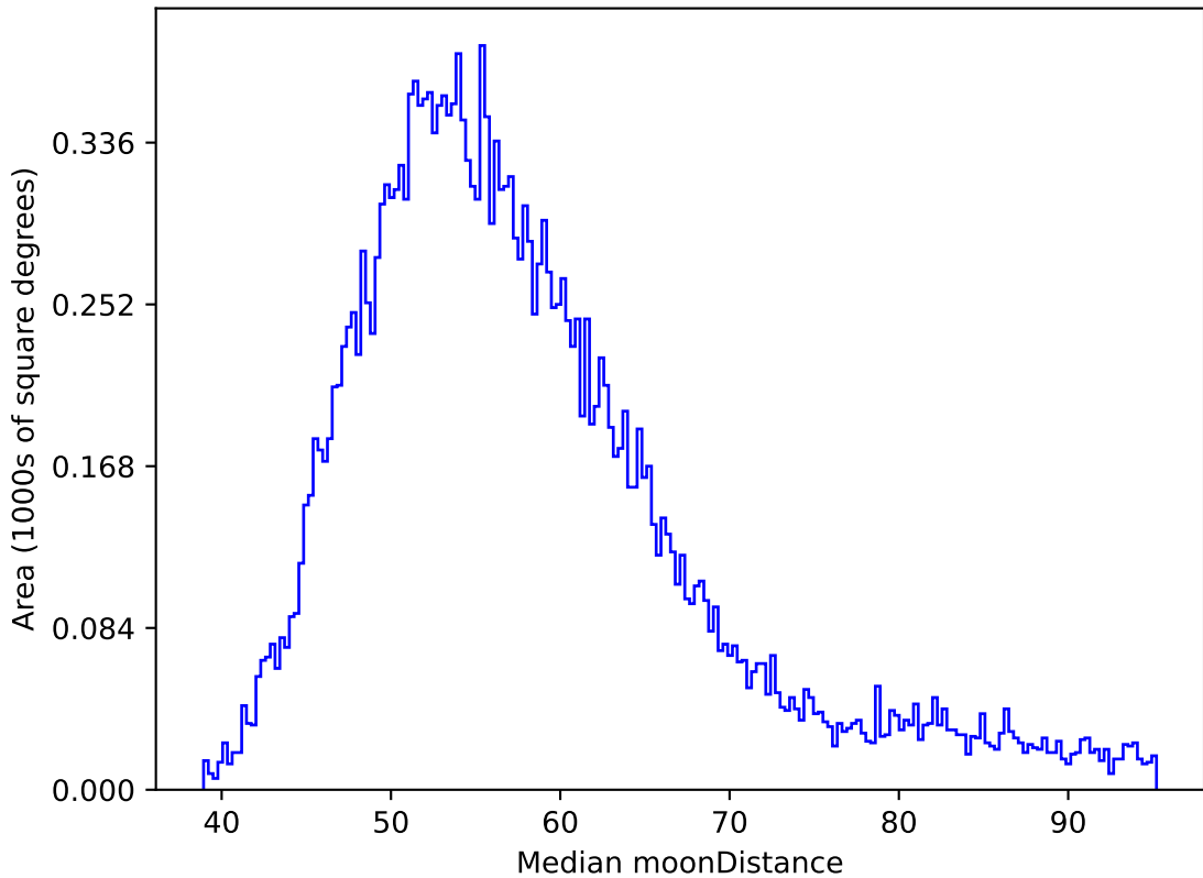
too_elab_r32_d2_ugrizy_v3.4_10yrs All sky y band: Median moonDistance
