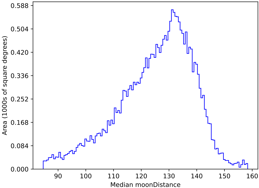
too_elab_r32_d2_ugrizy_v3.4_10yrs All sky u band: Median moonDistance
