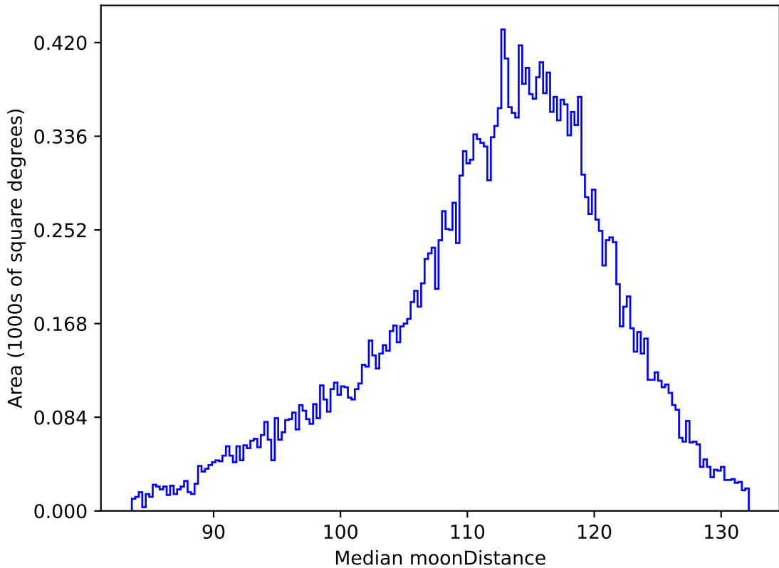
too_elab_r32_d2_ugrizy_v3.4_10yrs All sky r band: Median moonDistance
