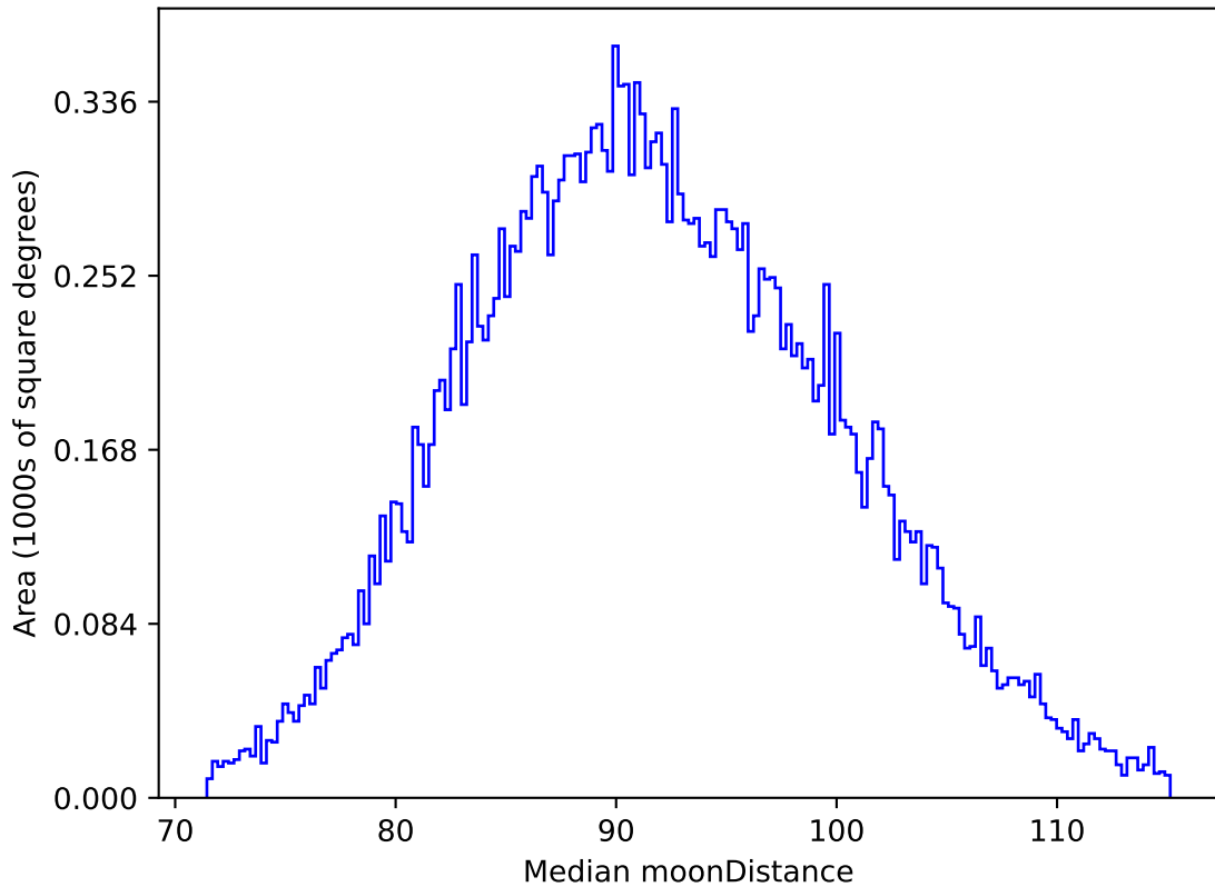
too_elab_r32_d2_ugrizy_v3.4_10yrs All sky i band: Median moonDistance
