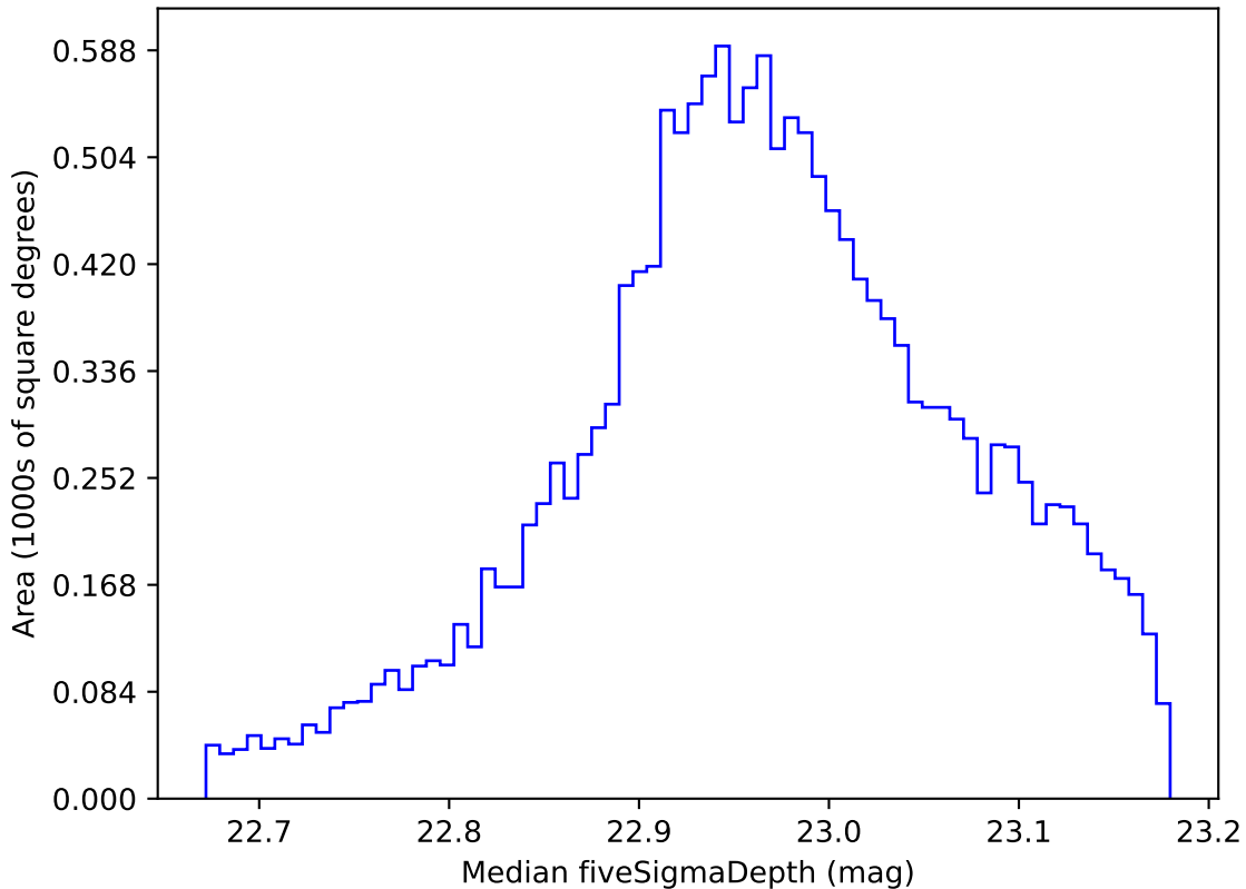
too_elab_r32_d2_ugrizy_v3.4_10yrs WFD z band: Median fiveSigmaDepth
