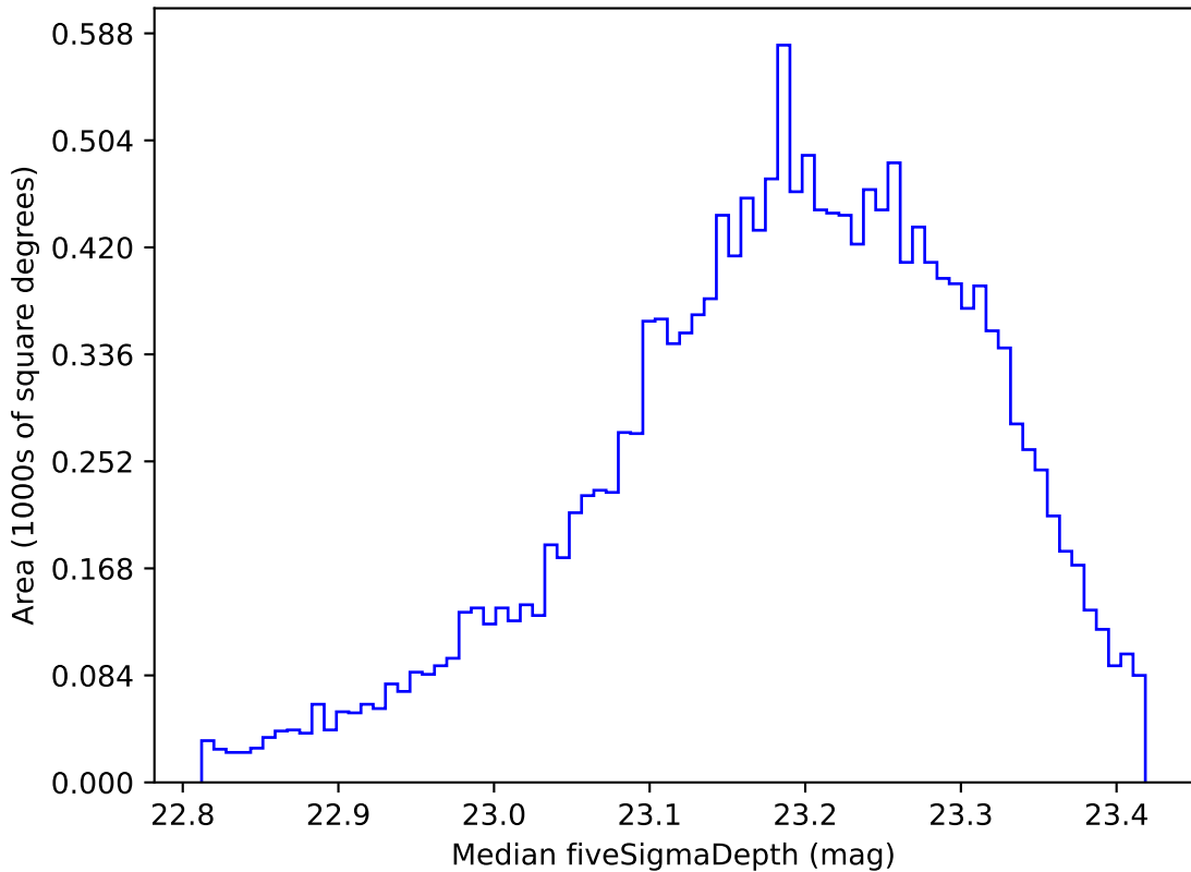
too_elab_r32_d2_ugrizy_v3.4_10yrs WFD u band: Median fiveSigmaDepth
