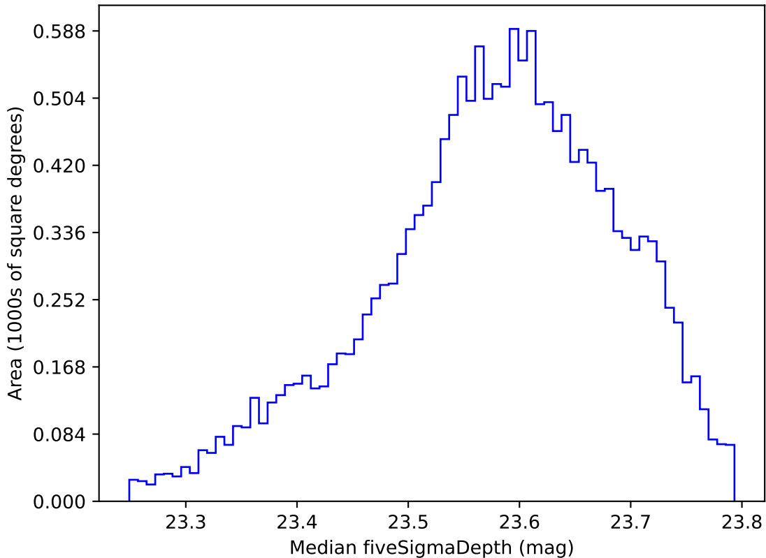
too_elab_r32_d2_ugrizy_v3.4_10yrs WFD i band: Median fiveSigmaDepth
