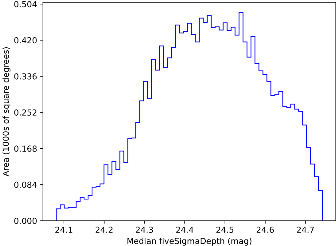
too_elab_r32_d2_ugrizy_v3.4_10yrs WFD g band: Median fiveSigmaDepth
