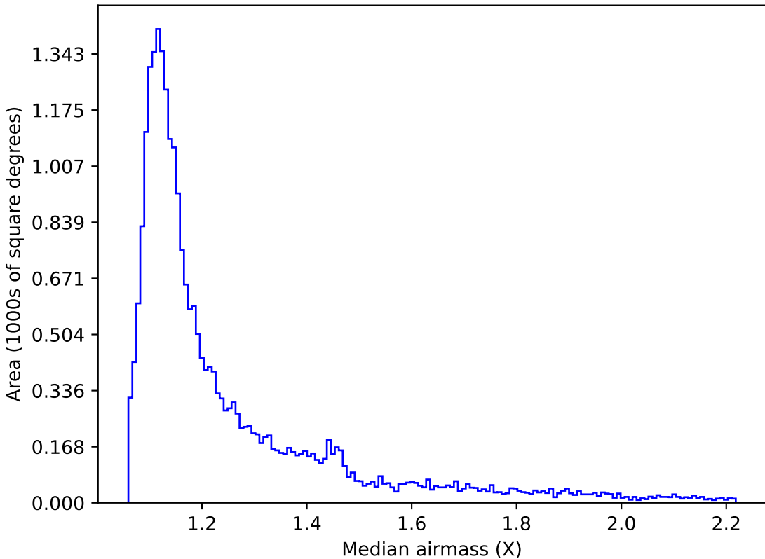
too_elab_r32_d2_ugrizy_v3.4_10yrs Yr 1 z band: Median airmass
