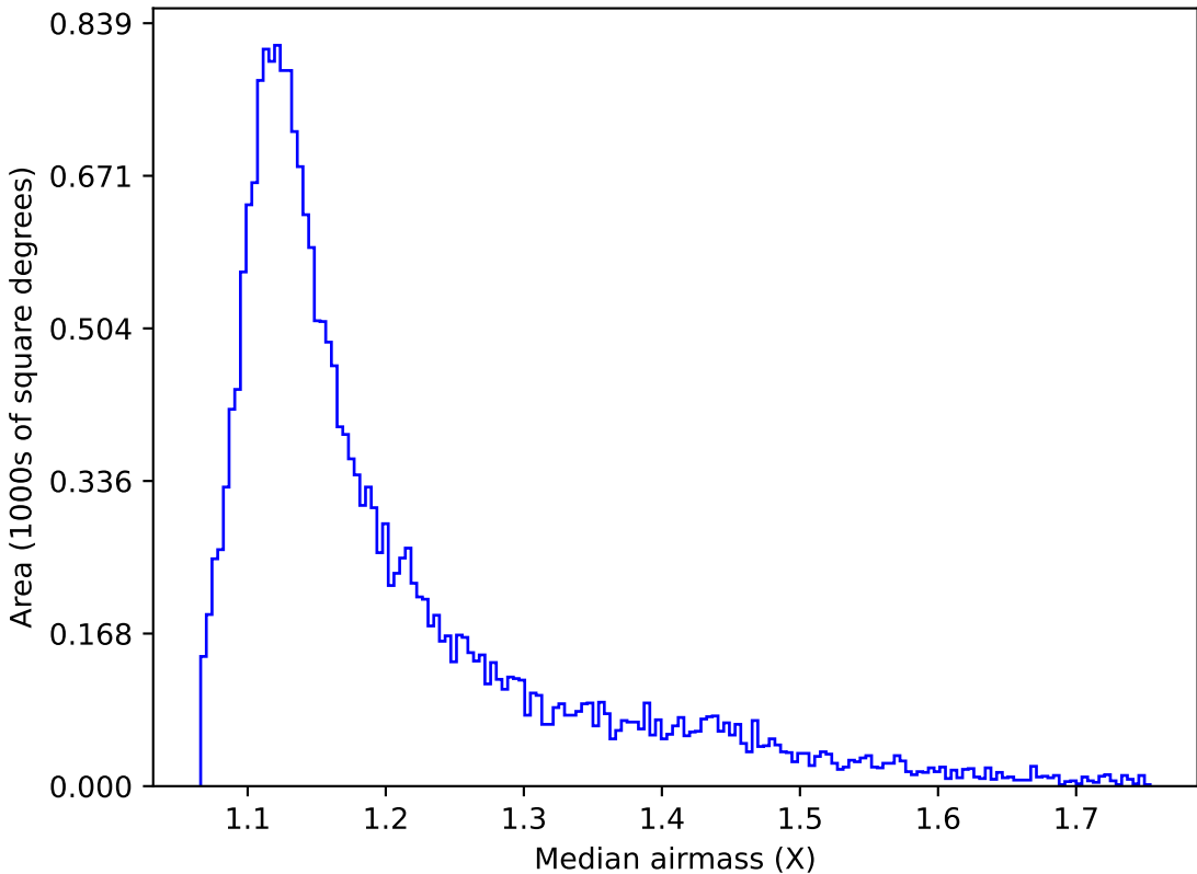
too_elab_r32_d2_ugrizy_v3.4_10yrs Yr 1 y band: Median airmass
